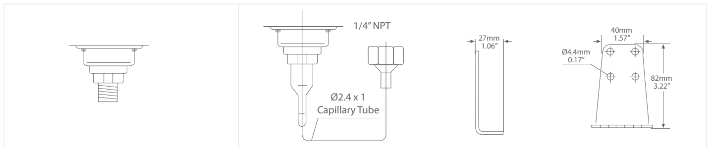
1/4" NPT CONNECTION
