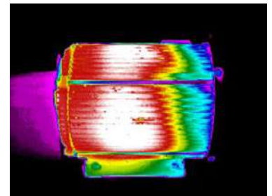
Infrared image of motor from Fluke TiS75+ thermal camera from 1.2 meters (4 feet) away
