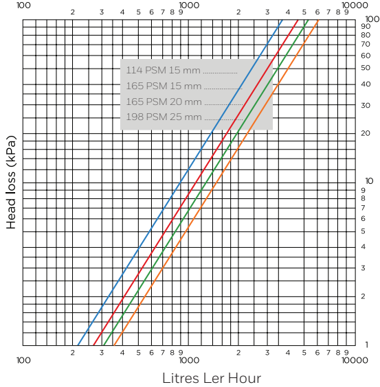
PRESSURE DROP GRAPH
