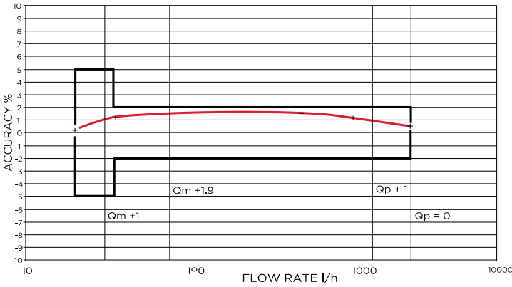
TYPICAL FLOW GRAPH
