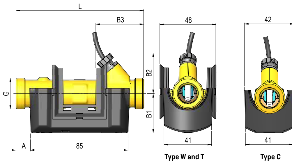
Flow sensor
