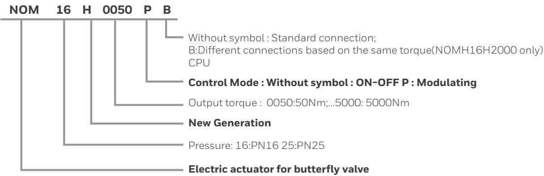
Matching table of butterfly valve and Electric actuator (Close-off pressure of below items:1000kpa)
